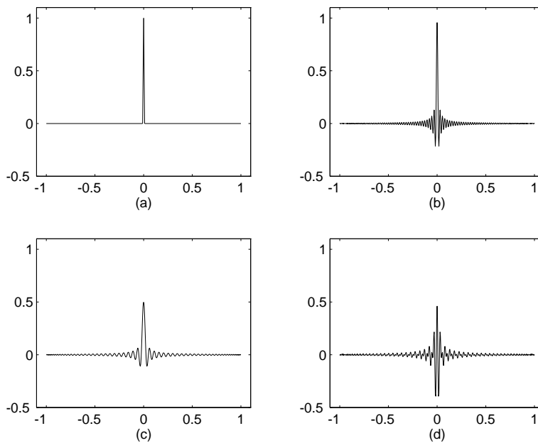
FIGURE 4. Decomposition with respect to w(t) = (1 - t^2)^{-1/2} for n = 128 . (a) Given function: f ; (b) projection on V_{2n} : f_{2n} ; decomposition: (c) f_n \in V_n ; (d) g_n \in W_n .
