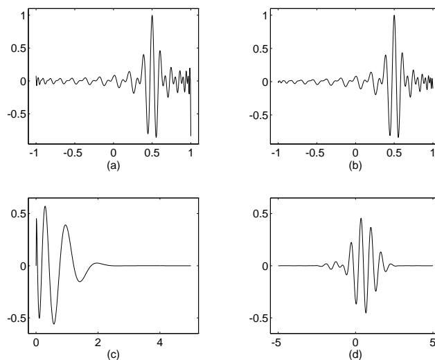
FIGURE 3. Various wavelets of degree n = 32 . (a) Legendre weight: w(t) = 1 ; \varphi_{32}(t; 0.5) ; (b) Jacobi weight: w(t) = (1-t)^{-0.5}(1+t)^{-0.8} ; \varphi_{32}(t; 0.5) ; (c) Laguerre weight: w(t) = t^{1/2} \exp(-t) ; \varphi_{32}(t; 1) \cdot w(t) ; (d) Hermite weight: w(t) = \exp(-t^2) ; \varphi_{32}(t; 1) \cdot w(t) .
