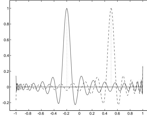
FIGURE 6. Scaling functions of degree n = 32 with respect to the Legendre weight w(t) = 1 and the parameter x_0^{(n+1)} = -0.2 (solid line) and x_1^{(n+1)} = 0.5 (dashed line).
