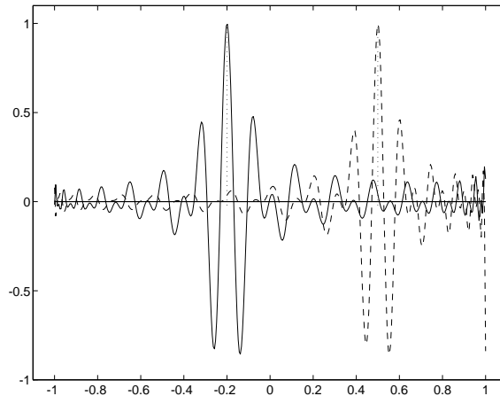
FIGURE 7. Wavelets of degree n = 32 with respect to the Legendre weight w(t) = 1 and the parameter z_0^{(n+1)} = -0.2 (solid line) and z_1^{(n+1)} = 0.5 (dashed line).
