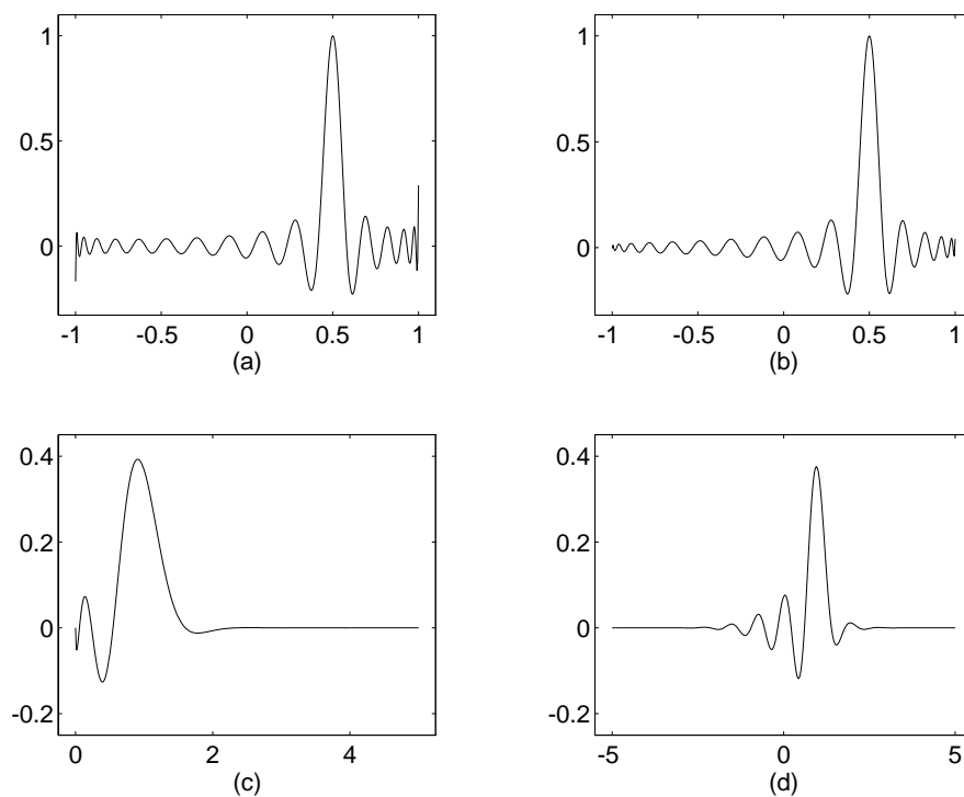
FIGURE 1. Various scaling functions of degree n = 32 . (a) Legendre weight: w(t) = 1; \varphi_{32}(t; 0.5) ; (b) Jacobi weight: w(t) = (1 - t)^{-0.5}(1 + t)^{-0.8}; \varphi_{32}(t; 0.5) ; (c) Laguerre weight: w(t) = t^{1/2} \exp(-t); \varphi_{32}(t; 1) \cdot w(t) ; (d) Hermite weight: w(t) = \exp(-t^2); \varphi_{32}(t; 1) \cdot w(t) .
