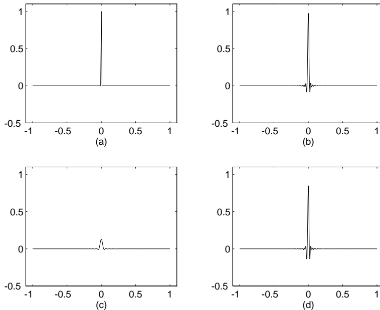
FIGURE 5. Decomposition with respect to w(t) = t^2(1 - t^2)^{-1/2} for n = 128 . (a) Given function: f ; (b) projection on V_{2n} : f_{2n} ; decomposition: (c) f_n \in V_n ; (d) g_n \in W_n .
