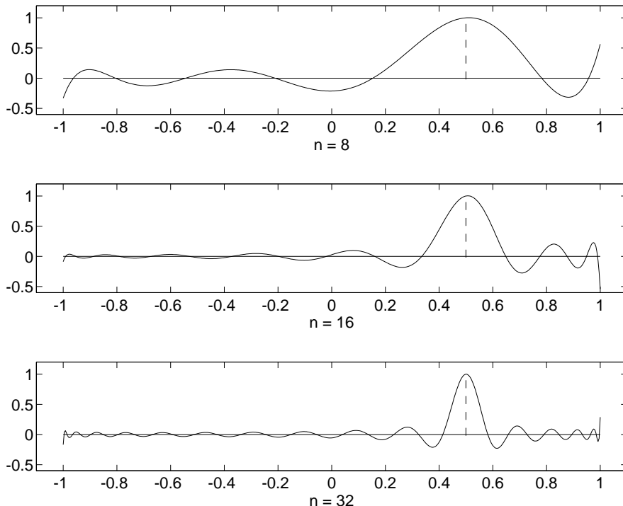
FIGURE 2. Scaling functions \varphi_n(t; 0.5) of degree n = 8, 16, 32 with respect to the Legendre weight w(t) = 1 and the parameter x_0^{(n+1)} = 0.5 .
