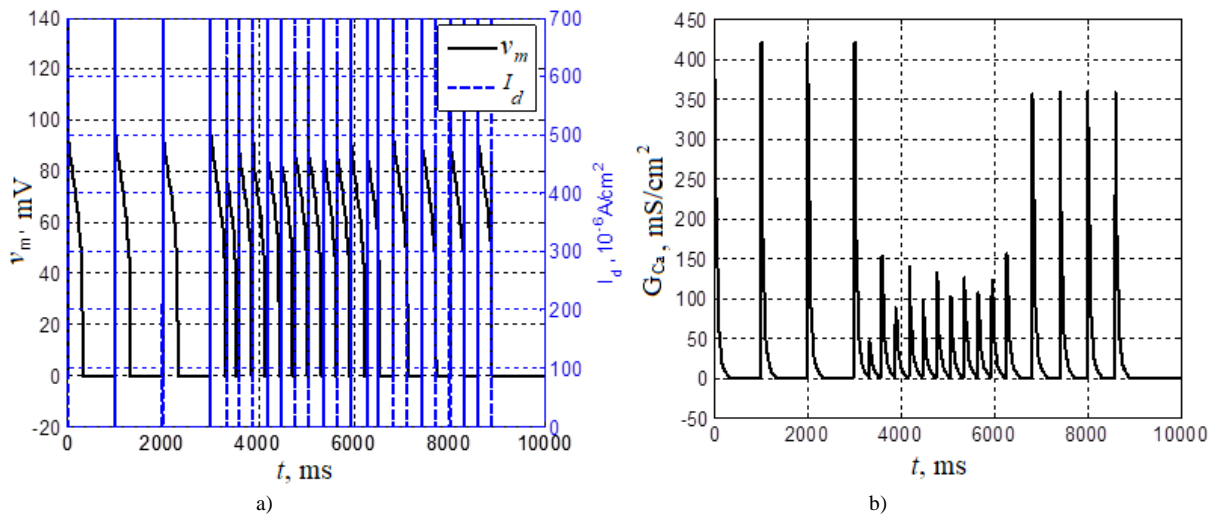
Fig.5. The switching from heart rhythm 1:1 to heart rhythm 2:1 in cardiomyocytes according to the initial delay of stimulation pulses (at delay DSP_1=280 ms and delay DSP_2=310 ms): action potentials (a); conductance of Ca^{2+} channels (b).
